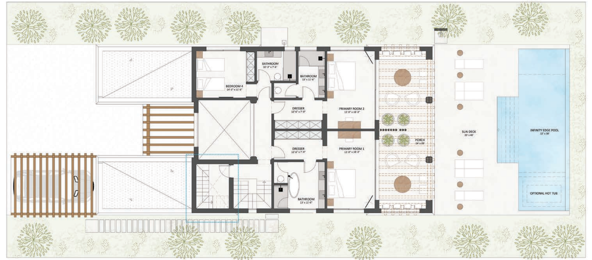
FIRST FLOOR
